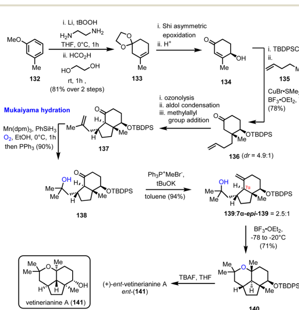
Scheme 14 Total synthesis of ent -vetiverianine A ( 141 ) (Sugita's group).
