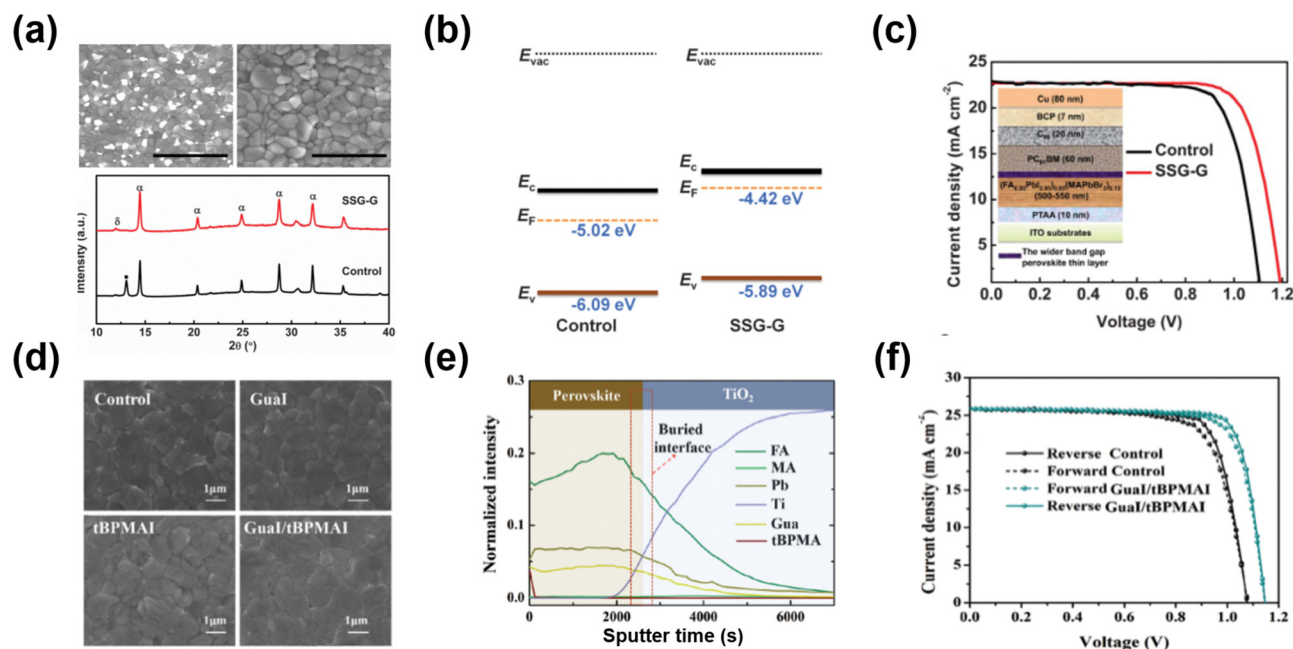
Fig. 10 (a) Top view SEM images of the perovskite film with/without GABr passivation (upper panel). XRD patterns (lower panel) of the perovskite film with/without GABr treatment (α: black perovskite phase; β: non-perovskite phase). (b) Schematic energy-level diagrams of the control and GABr-treated films. (c) J-V curves under the reverse scan of devices with/without GABr passivation. Reproduced with permission. 94 Copyright 2018, AAAS. (d) Top view SEM images of the perovskite film with/without binary GAI/tBPMAI treatment. (e) The time-of-flight secondary-ion mass spectrometry (ToF-SIMS) of the binary GAI/tBPMAI-treated perovskite film. (f) The forward/reverse scan J-V curves of the best devices with/without the binary GAI/tBPMAI treatment. Reproduced with permission. 95 Copyright 2021, Royal Society of Chemistry.
