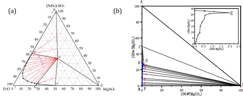
Fig. 16 (a) Ternary phase diagram of the ammonium sulphate, magnesium sulphate and water system at 25 °C. The letters in the diagram represents the coexisting solids in the supersaturated solution: A represents the equilibrium \text{MgSO}_4\text{-H}_2\text{O} , B shows the solubility of \text{MgSO}_4 , at C two main solids were identified \text{MgSO}_4\cdot x\text{H}_2\text{O} and \text{MgSO}_4\cdot (\text{NH}_4)_2\text{SO}_4\cdot 6\text{H}_2\text{O} , D shows the precipitation of only \text{MgSO}_4\cdot (\text{NH}_4)_2\text{SO}_4\cdot 6\text{H}_2\text{O} , the E, F, and I indicates 100% or the represented phases in the triangle vertices, G shows the solubility of (\text{NH}_4)_2\text{SO}_4 , and H corresponds to (\text{NH}_4)_2\text{SO}_4 and \text{MgSO}_4\cdot (\text{NH}_4)_2\text{SO}_4\cdot 6\text{H}_2\text{O} (Liu et al., Copyright© 2018, American Chemical Society). 139 (b) Equilibrium phase diagram of the ternary diagram of \text{MgCO}_3\text{-MgSO}_4\text{-H}_2\text{O} system at 25 °C. A and B represents pure \text{MgSO}_4 and pure \text{MgCO}_3 , respectively, C and D shows the solubility of \text{MgSO}_4\cdot 7\text{H}_2\text{O} and \text{MgCO}_3 , respectively, and at point E, epsomite and magnesite co-precipitate, F is the solubility of \text{MgCO}_3 (0.021%) (Li et al., Copyright © 2021, American Chemical Society). 140
