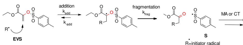
Fig. 13 AFCT mechanism for an ethyl ester activated vinyl sulfone ester (EVS).
