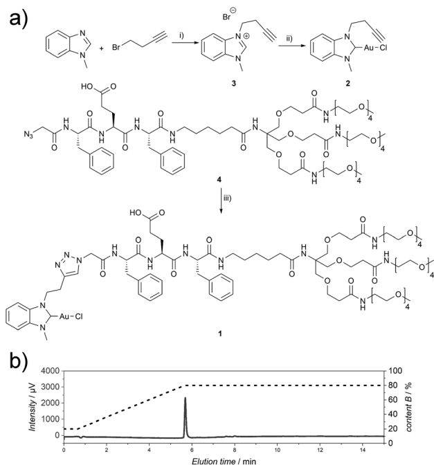
Fig. 1 (a) Synthetic route for the synthesis of compound 1 . (i) 1-Methyl-1H-benzod[e]imidazole (1.0 eq.), 4-bromobut-1-yne (1.5 eq.), toluene, 110 °C, 72 h; (ii) (1) 3 (1.0 eq.), Ag 2 O (0.6 eq.), DCM, r.t., 68 h, (2) Au(I)Cl (tht) (1.0 eq.), NaCl (1.5 eq.), r.t., 2.5 h; (iii) 2 (1.1 eq.), 4 (1.0 eq.), CuSO 4 ·5H 2 O (0.2 eq.), TBTA (0.2 eq.), sodium L-ascorbate (0.2 eq.), THF:H 2 O, 1:1, 45 °C, 7 h. (b) Analytical HPLC chromatogram (215 nm) of 1 (CH 3 CN:H 2 O gradient, 1 mM NH 4 HCO 3 ).
