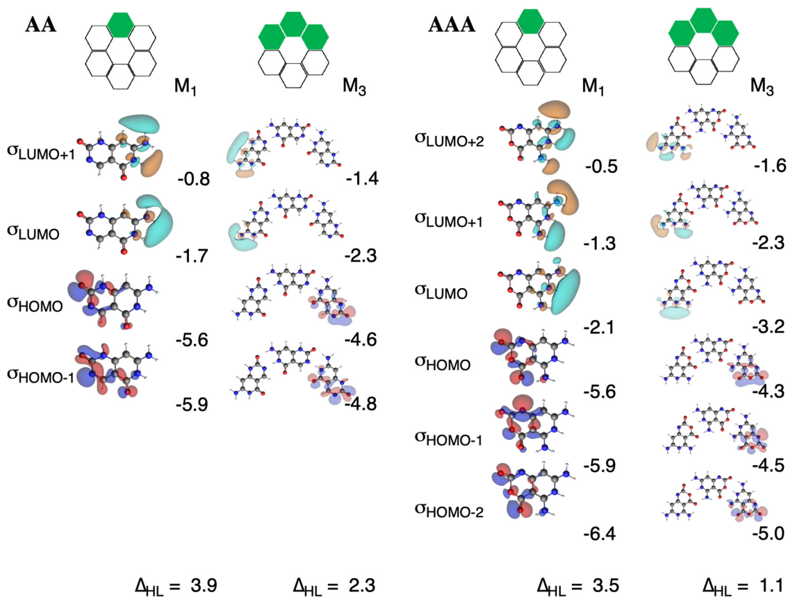
Fig. 9 N–H unoccupied \sigma_{LUMO} orbitals and oxygen and nitrogen lone-pair \sigma_{HOMO} orbitals of the front atoms of AA (left) and AAA (right) and their corresponding energies (in eV) for stepwise M 1 and M 3 states, computed at the ZORA-BLYP-D3(BJ)/TZ2P level. The HOMO–LUMO gap ( \Delta_{HL} , in eV) is also included.
