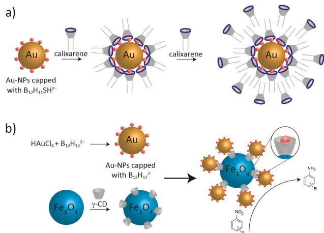
Fig. 10 (a) Assembly of a calixarene derivative on B_{12}H_{11}SH^{2-} coated AuNPs. 41 (b) The preparation of B_{12}H_{12}^{2-} -capped gold nanoparticles and CD-functionalized Fe_3O_4 and their assembly as a catalyst for the reduction of nitroaromatics. 166
