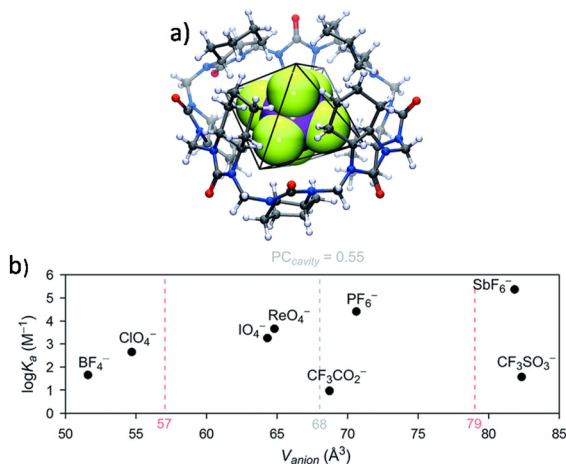
Fig. 6 (a) Crystal structure of the cyclohexanohemicucurbit[8]uril-SbF 6 - complex. (b) Binding affinities (log K a ) of large anions to cyclohexanohemicucurbit[8]uril as a function of the anion volume ( V anion ). Note the clear trend of increasing affinity with the anion size when the two perfluorinated organic ions at the bottom are excluded. Reproduced from ref. 123 with permission from the Royal Society of Chemistry.
