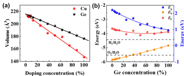
Fig. 9 (a) Normalized volumes of Ge- and Cu-doped bulk \text{CsPbBr}_3 . (b) Bandgap coupled to the energies of the VBM and the CBM for \text{CsPb}_{1-x}\text{Ge}_x\text{Br}_3 . Reproduced from ref. 81 with permission from the American Chemical Society. Copyright 2021.
