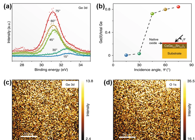
Fig. 10 (a) Ge 3d XPS spectra at different incidence angles in a vapor-deposited \text{CsSn}_{0.5}\text{Ge}_{0.5}\text{I}_3 film. (b) The corresponding plot of the Ge(II) fraction vs. the incidence angle. (c) and (d) XPS maps of Ge 3d (33 eV) and O 1s (532 eV). Reproduced from ref. 82 with permission from Springer Nature. Copyright 2020.
