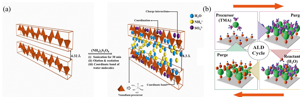
Fig. 1 A schematic of the preparation of AVNF and \text{Al}_2\text{O}_3/\text{Zn} . (a) A scheme for the synthesis of ammonium vanadate nanofiber (AVNF: (\text{NH}_4)_2\text{V}_6\text{O}_{16} \cdot 1.5\text{H}_2\text{O} ) from \text{V}_2\text{O}_5 using the sonochemical method. (b) A scheme for the deposition of \text{Al}_2\text{O}_3 formed by the reaction of TMA (trimethylaluminum, \text{Al}(\text{CH}_3)_3 ) and distilled water ( \text{H}_2\text{O} ) in an ALD cycle.
