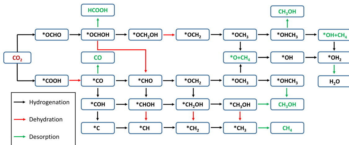
Scheme 1 Schematic representation of multiple pathways of electrochemical reduction of \text{CO}_2 to C1 products on the \text{MoS}_2 monolayer with embedded Cu. Red and green arrows are used to distinguish the significant steps, namely dehydration and desorption, respectively.
