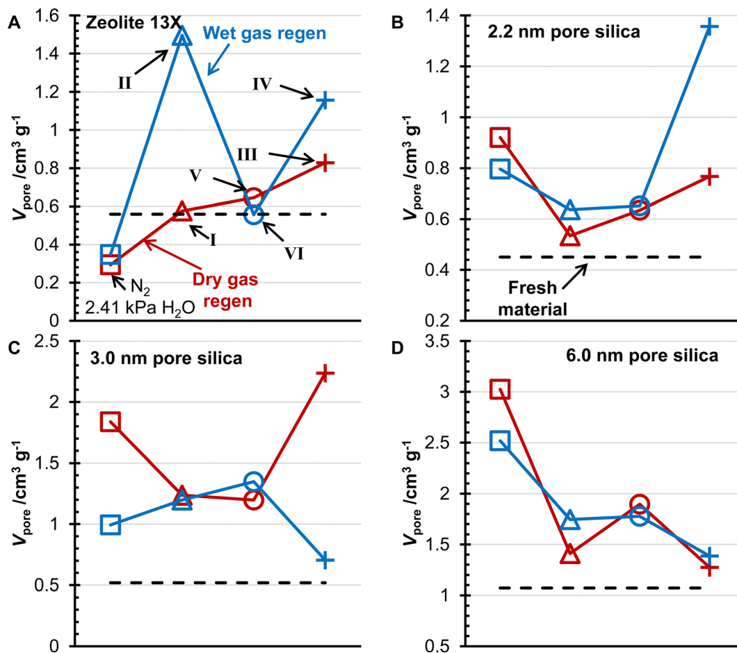
Fig. 7 The pore volumes of zeolite 13X (A), 2.2 nm pore size silica (B), 3.0 nm pore size silica (C), and 6.0 nm pore size silica (D) for the three gas mixtures ( p_{\text{CO}_2} = 3.49 kPa, p_{\text{H}_2\text{O}} = 2.39 kPa, \Delta ; p_{\text{CO}_2} = 3.49 kPa, p_{\text{H}_2\text{O}} = 2.21 kPa, \circ ; p_{\text{CO}_2} = 34.9 kPa, p_{\text{H}_2\text{O}} = 2.21 kPa, + ) and the previously published results ( p_{\text{H}_2\text{O}} = 2.41 kPa, \square ) without \text{CO}_2 . 20 Results for dry gas (red) and wet gas (blue) regeneration conditions are reported. The solid black line represents the surface area of the fresh material.
