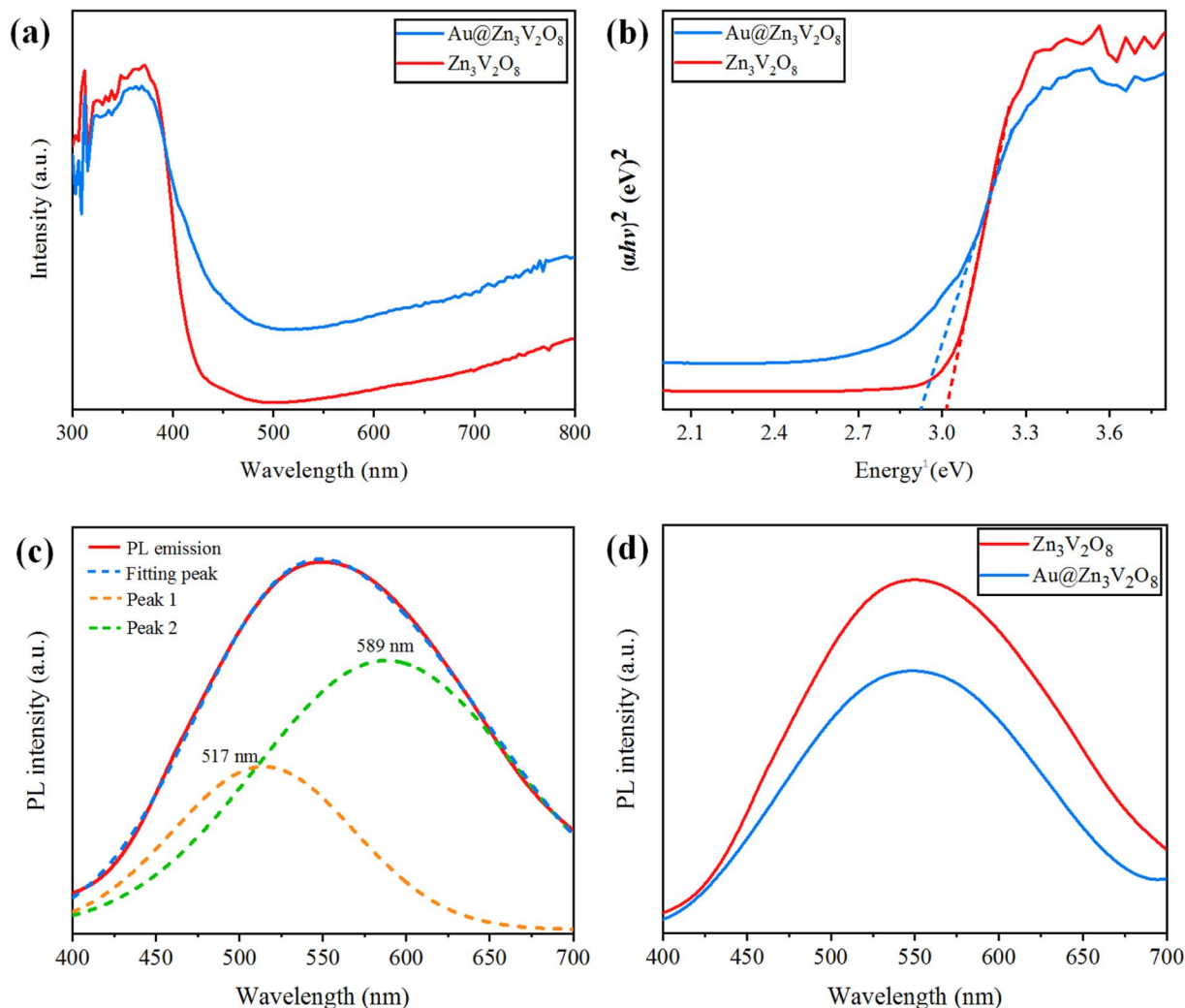
Fig. 6 (a) UV-Vis-DRS, (b) energy curves (eV), (c) PL emission spectra and fitting of the peaks, and (d) PL emission spectra for the \text{Zn}_3\text{V}_2\text{O}_8 and \text{Au@Zn}_3\text{V}_2\text{O}_8 catalysts.
