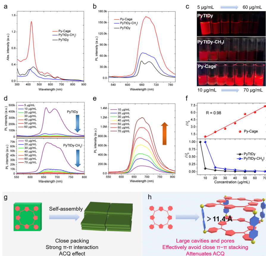
Fig. 2 UV-vis absorption spectra (a) and fluorescence (PL) spectra (b) of the Py-Cage, PyTtDy-CH 3 I, and PyTtDy ( 10 \mu\text{g mL}^{-1} ) in H 2 O/DMSO ( v_{\text{water}}/v_{\text{DMSO}} = 99:1 ) mixture solvent. (c) Photographs of the Py-Cage, PyTtDy-CH 3 I, and PyTtDy in aqueous solution (1% DMSO) at different concentrations under UV light at 365 nm. Fluorescence spectra of aqueous solutions of PyTtDy (d, top), PyTtDy-CH 3 I (d, bottom) and the Py-Cage (e) with different concentrations. (f) The fluorescence intensity changes of the Py-Cage, PyTtDy-CH 3 I, and PyTtDy with increasing concentration. (g) and (h) Schematic comparison between traditional planar porphyrin-based photosensitizers and the porous porphyrin nanocage in attenuating the ACQ effect.
