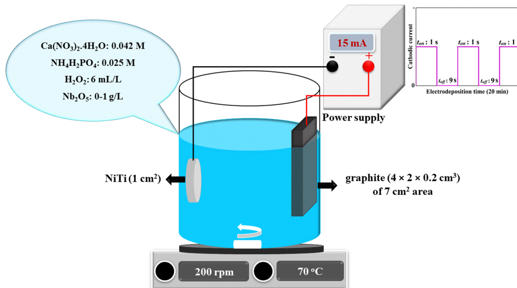
Fig. 1 Schematic illustration of the electrolyte composition and electroplating parameters in the present work.
