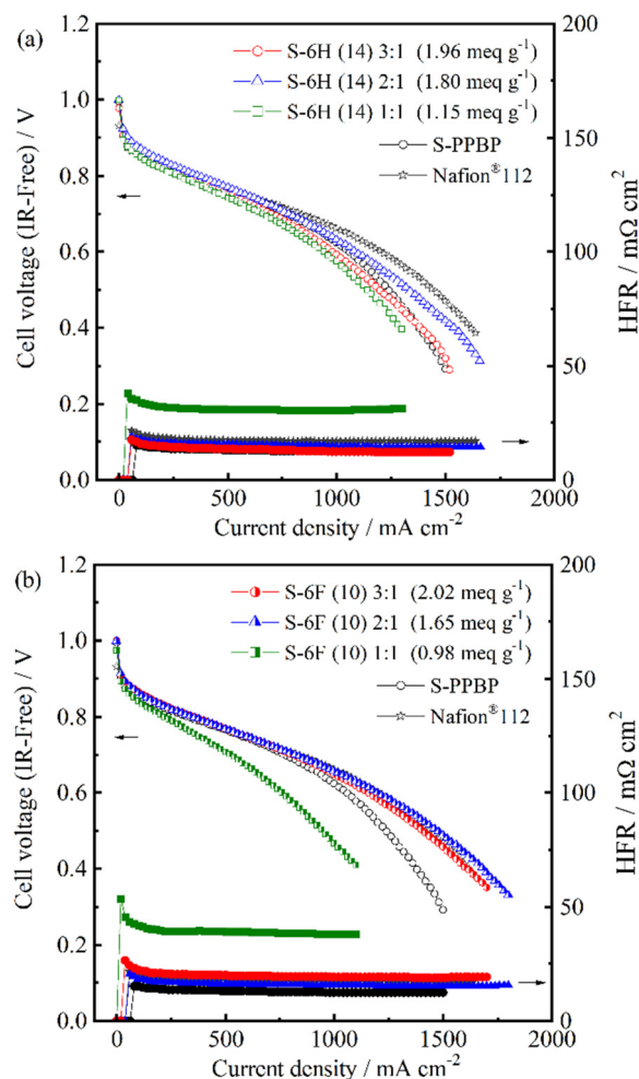
Fig. 11 IR-free cell voltage and HFR as a function of current density for a 5 cm 2 -sized PEFC with H 2 (500 mL min -1 , 0.1 MPaG) and air (1000 mL min -1 , 0.1 MPaG) feeds for (a) S-6H and (b) S-6F membranes at 80 °C and 100% RH.
