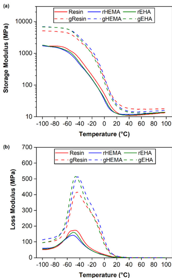
Fig. 6 DMA of printed specimens under single cantilever mode at 1 Hz. (a) storage modulus ( E' ) and (b) loss modulus ( E'' ).
