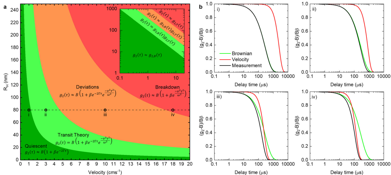
Fig. 8 (a) Regions of the approaches required to analyse under flow DLS data for a range of flow velocities (0–20 \text{cm s}^{-1} ) and R_H (<250 nm) with boundaries defined by green: 1 > g_{2,\tau}(\tau_q) > 0.98 , light green: 0.98 > g_{2,\tau}(\tau_q) > 0.75 , orange: 0.75 > g_{2,\tau}(\tau_q) > 0.02 , red: 0.02 > g_{2,\tau}(\tau_q) using the parameters: \theta = 130^\circ , \lambda = 638 nm, T = 25 °C, refractive index n = 1.33 , \eta = 8.9 \times 10^{-4} Pa s (water), beam radius \omega = 25 \mu\text{m} . (b) The theoretical Brownian exponential decay (green line) and velocity Gaussian (red line) contributions to the overall measured correlogram (black lines) calculated at the marked regions (i–iv) in panel a using the above mentioned instrument parameters.
