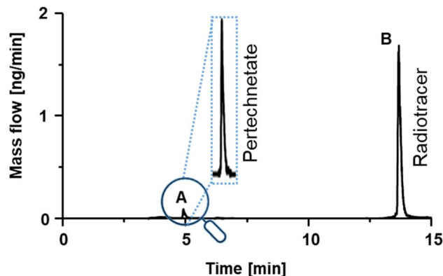
Fig. 3 ^{99}\text{Tc} mass flow chromatogram of experimental radiotracer Tc-MEA223. Two different signals could be detected and calibrated.
