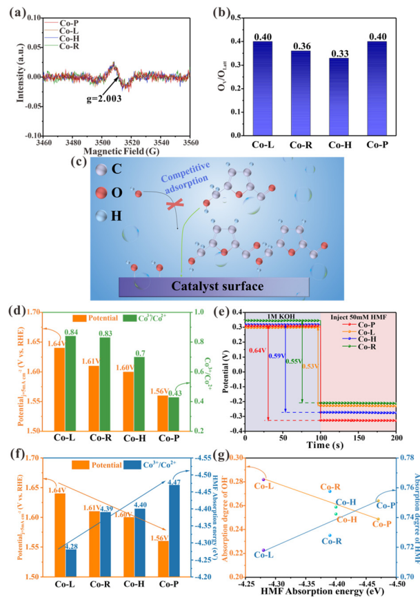
Fig. 3 (a) EPR spectra of Co-R, Co-L, Co-H and Co-P. (b) The O_v/O_{Latt} ratio of Co-R, Co-L, Co-H and Co-P from XPS spectra. (c) Competitive adsorption between HMF and OH^- from the schematic. (d) Histogram showing the correlation between Co^{3+}/Co^{2+} ratio from XPS spectra and HMF electrooxidation activity. (e) OCP curves of Co 3 O 4 NCs in 1.0 M KOH and 50 mM HMF was injected subsequently. (f) Histogram showing the correlation between adsorption energy on Co 3 O 4 NCs and HMF electrooxidation activity. (g) Adsorption degree of OH^- and HMF on Co 3 O 4 NCs as HMF adsorption energy rises.
