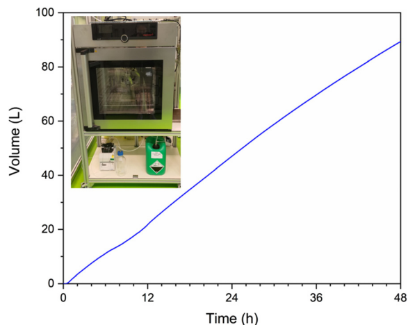
Fig. 7 Cumulative \text{H}_2 volume generated in continuous reactor by cobalt chitosan spheres over a 48 h period. Measurements taken once per second using mass flow meters. The inset shows a photo of the system with the fuel vat, pump, reactor oven and waste vat. A detailed description of the reactor system is included in the ESI†
