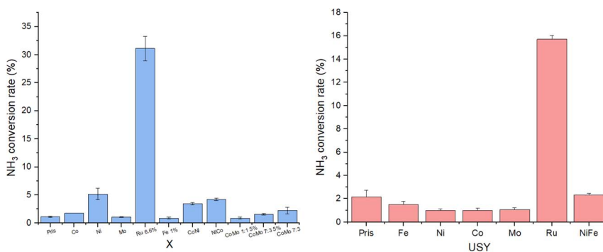
Fig. 14 \text{NH}_3 conversion rates of monometallic and bimetallic catalysts supported on X and USY at reaction conditions of 450 °C and 30 000 WHSV with pure ammonia feed gas. All metals were loaded in a M : Al ratio of 1 : 1, including each component of bimetallic catalysts, unless its wt% loading is given instead. Ratios for CoMo catalysts reflect Co : Mo ratio.
