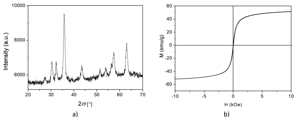
Fig. 1 a) X-ray diffraction spectrum of the as-prepared MNPs; b) magnetization vs. magnetic field at 293 K.
