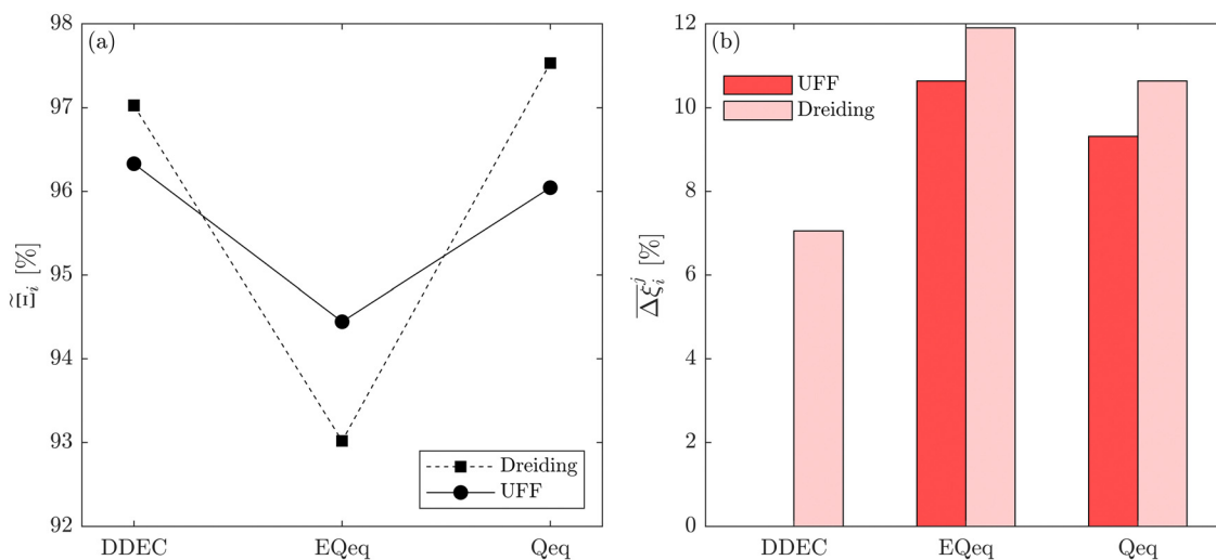
Fig. 10 Process-level uncertainty metrics for CO 2 purity-recovery optimisations. (a) Pareto-dominance plot constructed from \tilde{\epsilon}_i values using the CRAFTED-u dataset. (b) Average hypervolume error, \Delta \tilde{\epsilon}_i , between i = \text{UFF} + \text{DDEC} and other molecular forcefields ( j \neq \text{UFF} + \text{DDEC} ) for the CRAFTED-u dataset. Higher values of \Delta \tilde{\epsilon}_i indicate a larger average uncertainty with the UFF + DDEC baseline.
