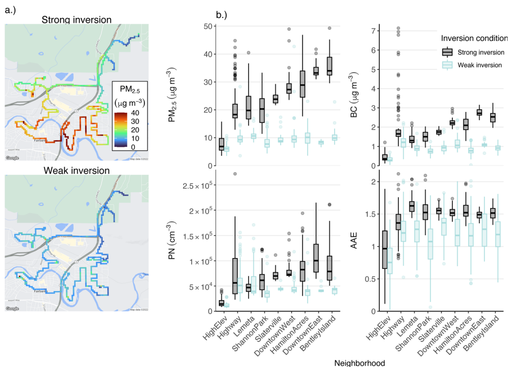
Fig. 5 (a) PM 2.5 map for strong and weak inversion conditions using 50 m grid cell aggregations. Concentration values outside of the colorscale range are given the end values of the range, for visualization purposes. (b) Neighborhood boxplots of PM 2.5 , BC, PN, and AAE for both inversion conditions. Neighborhoods for all pollutants are arranged on the x-axis in order of increasing median PM 2.5 concentration within the strong inversion category.
