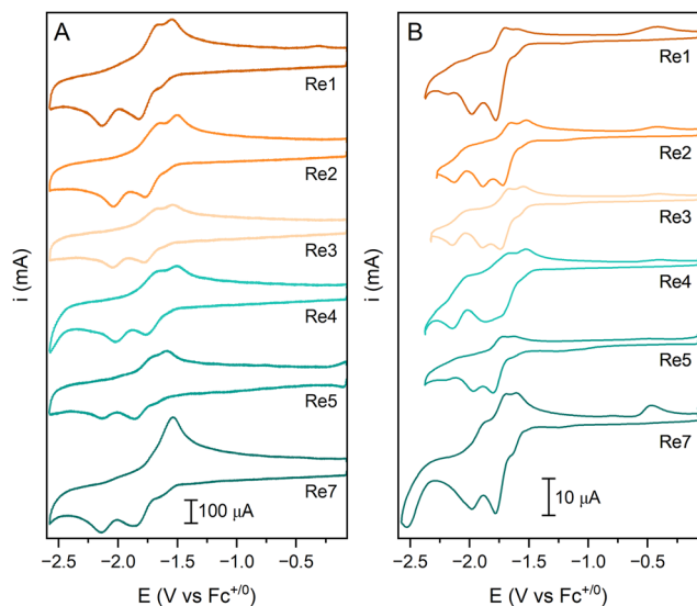
Fig. 6 Cyclic voltammograms of Re1–5 and Re7 recorded in acetonitrile under N_2 at scan rates (A) 10 V s^{-1} and (B) 0.1 V s^{-1} (supporting electrolyte 0.1 M n -Bu 4 NBF 4 ). Re7 is shown for comparison.
