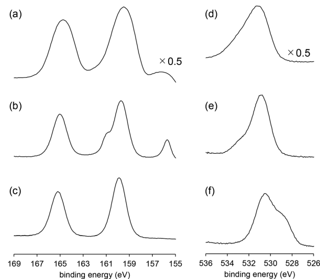
Fig. 7 XPS (a–c) Bi 4f and (d–f) O 1s spectra of \text{BiPO}_4 -DEG. (a and d) \text{BiPO}_4 -DEG at room temperature under evacuation, (b and e) \text{BiPO}_4 -DEG at 550 °C under evacuation, and (c and f) \text{BiPO}_4 -DEG at 550 °C under \text{O}_2 (0.1 mbar).
