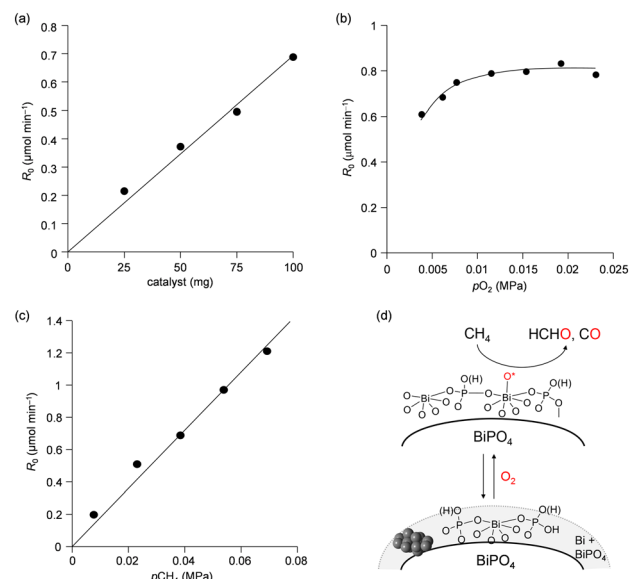
Fig. 6 Effect of (a) catalyst amount and partial pressure of (b) \text{O}_2 and (c) \text{CH}_4 on reaction rate. Reaction conditions for (a): \text{BiPO}_4 -DEG (25–100 mg), \text{CH}_4/\text{O}_2/\text{N}_2 (5/1/7 sccm; total 13 sccm), reaction temperature (550 °C). Reaction conditions for (b): \text{BiPO}_4 -DEG (100 mg), \text{CH}_4/\text{O}_2/\text{N}_2 (5/0.5–3/7.5–5 sccm; total 13 sccm), reaction temperature (550 °C). Reaction conditions for (c): \text{BiPO}_4 -DEG (100 mg), \text{CH}_4/\text{O}_2/\text{N}_2 (1–9/1/11–3 sccm; total 13 sccm), reaction temperature (550 °C). (d) Proposed reaction mechanism for oxidation of \text{CH}_4 with \text{O}_2 over \text{BiPO}_4 -DEG.
