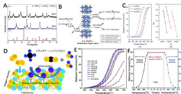
Fig. 9 (A) XRD patterns of Mn1, Mn2, and Mn3 catalysts. Reproduced from ref. 170 with permission from Elsevier. (B) Proposed mechanism of oxygen transfer on the \text{La}_{n+1}\text{Ni}_{n-1}\text{O}_{3n+1} layered perovskites in catalytic oxidation of toluene and methane; (C) conversion rates and Arrhenius plots of \text{La}_2\text{NiO}_4 (□), \text{La}_4\text{Ni}_3\text{O}_{10} (○), and \text{LaNiO}_3 (Δ) in methane oxidation. Condition: methane (1 vol%), \text{O}_2 (10 vol%), 0.5 g catalyst, GHSV = 19 200 \text{mL g}^{-1} \text{h}^{-1} . Reproduced from ref. 171 with permission from the American Chemical Society. (D) Schematic representation of the catalytic methane oxidation on the \text{Y}_x\text{InO}_{3+\delta} catalyst; (E) methane conversion as a function of temperature over the YIO- x catalysts; (F) the stability test performed at 700 °C within 50 h under 1% vol. \text{CH}_4 , 10% vol. \text{O}_2 in nitrogen; GHSV = 30 000 \text{mL g}^{-1} \text{h}^{-1} . Reproduced from ref. 172 with permission from the Royal Society of Chemistry.
