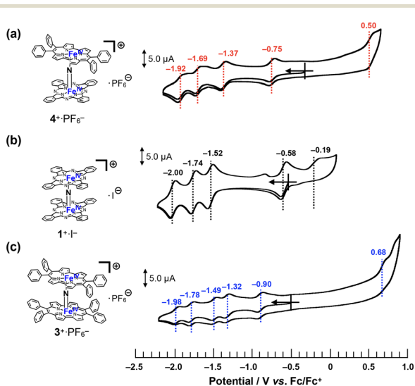
Fig. 5 Comparison of cyclic voltammograms of (a) 4^+\cdot\text{PF}_6^- , (b) 1^+\cdot\text{I}^- , and (c) 3^+\cdot\text{PF}_6^- in a pyridine solution containing 100 mM of ^n\text{Bu}_4\text{N}^+\text{PF}_6^- at room temperature. [Substrate] = 200 \mu\text{M} , [scan rate] = 100 \text{mV s}^{-1} .
