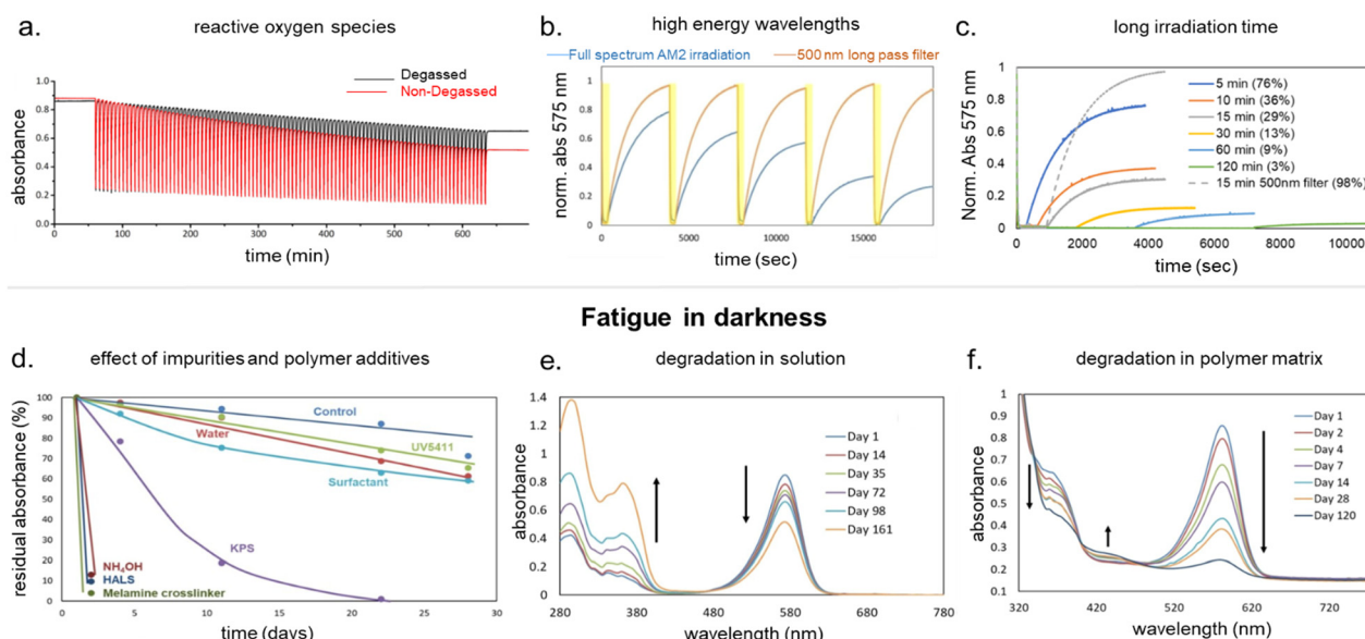
Fig. 18 Mechanisms of DASA fatigue in presence of light irradiation and in darkness. (a) Fatigue measurements of a barbituric acid-based first-generation DASA measured by UV-Vis spectroscopy at 565 nm under atmospheric conditions (red) and degassed with argon (black). After 100 cycles of 45 sec irradiation (567 nm) followed by 5 min equilibration in the dark, the degassed sample decomposed by 25%, while the non-degassed sample decomposed by 41%. Figure adapted with permission from ref. 35 Copyright Royal Society of Chemistry 2018. (b) Repetitive photo-cycling of a second-generation DASA based on N -methyl aniline and 1,3-dimethylbarbituric acid in a solid polymer matrix (PBA-co-PMMA; 2 wt%) by irradiation with an AM2 solar simulated light (blue) and in presence of a 500 nm long pass filter (orange). (c) Photoswitching of a second-generation DASA based on N -methyl aniline and 1,3-dimethylbarbituric acid in a polymer matrix (poly( tert -butyl methacrylate)-co-PBA; 2 wt%) after different irradiation times with an AM2 solar simulated light directly and in presence of a 500 nm long pass filter. The light exposure time was found to decrease the thermal recovery to the DASA open isomer (recovery percentage is given in brackets). (d) Residual open isomer absorbance of a second-generation DASA based on N -methyl aniline and 1,3-dimethylbarbituric acid at dark equilibrium overtime in acetonitrile (0.15 mM) in presence of different impurities at 0.2 wt% (UV5411: common UV absorber based on benzotriazole; KPS: potassium persulfate; HALS: hindered amine light stabilizer). (e) Decomposition of a second-generation DASA based on N -methyl aniline and 1,3-dimethylbarbituric acid in acetonitrile (0.15 mM) stored in the dark over time. A decrease in the open isomer absorbance band at 575 nm and an increase in absorbance in the UV region (370 nm) could be observed. The latter changes are likely caused by the retro formation of the furan adduct. (f) Decomposition of a second-generation DASA based on N -methyl aniline and 1,3-dimethylbarbituric acid within a solid polymer matrix (PBA-co-PMMA; 2 wt%) over time stored in darkness. An increase of absorbance band at 430 nm, and decrease at 370 nm and 585 nm is observed. Figures adapted with permission from ref. 138 Copyright 2023 Elsevier.
