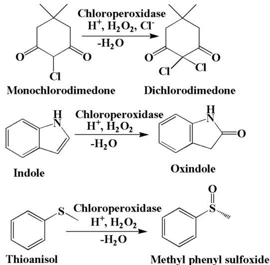
Fig. 23 Biocatalytic reactions catalyzed by chloroperoxidase.
