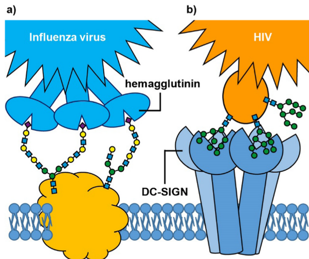
Fig. 1 Glycan-mediated cell targeting: (a) influenza virus hemagglutinin binds to multiple sialic acids on cell surface glycoproteins; (b) cell surface DC-SIGN receptor binds to mannoseglycans on the surface of HIV.
