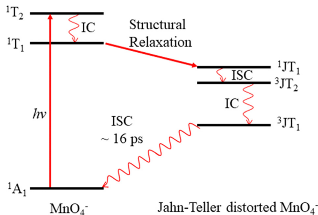
Fig. 1 Excitation of \text{MnO}_4^- in the visible to 1^1T_2 , followed by rapid relaxation via the 3^1JT_1 state of a Jahn–Teller distorted \text{MnO}_4^- back to 1^1A_1 , via structural relaxation, internal conversion (IC) and intersystem crossing (ISC). The transition from 1^1A_1 to 1^1T_1 is symmetry forbidden.
