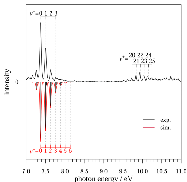
Fig. 5 Experimental threshold photoelectron spectrum of SiF in the vicinity of the X^+1\Sigma^+ \leftarrow X^2\Pi photoionising transition (in black) compared with our harmonic Franck–Condon calculation convolved with a Gaussian line shape (FWHM = 40 meV) at a vibrational temperature of 600 K (in red). The above red assignment corresponds to our harmonic calculation whereas the black comb follows the anharmonicity which allows an unambiguous attribution of the ionising transitions towards v^+ = 20 –25 (observed through autoionisation). See the text for details.
