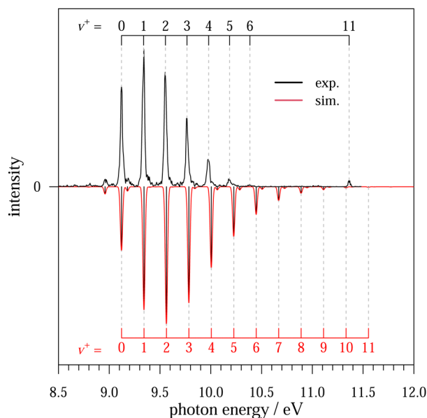
Fig. 2 Experimental threshold photoelectron spectrum of CF in the vicinity of the X^+ \ ^1\Sigma^+ \leftarrow X \ ^2\Pi photoionising transition (in black) compared with our harmonic Franck–Condon calculation convolved with a Gaussian line shape (FWHM = 26 meV) at a vibrational temperature of 600 K (in red). The red assignment corresponds to our harmonic calculation whereas the black comb follows the anharmonicity which allows an unambiguous attribution of the ionising transition towards v^+ = 11 (observed through autoionisation). See the text for details.
