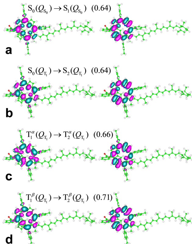
Fig. 6 NTOs most representative of the indicated electronic excitations (their weights are provided in parentheses) of the ortho -carotenoporphyry molecular dyad in THF-like solvent, represented using an iso-value of 0.02. Lobes of different signs are drawn in different colors. This distinction is used for better visualization but is clearly irrelevant for describing the degree of MO similarity. The MOs were rendered using the gOpenMol 3.00 molecular visualization program. 71,72
