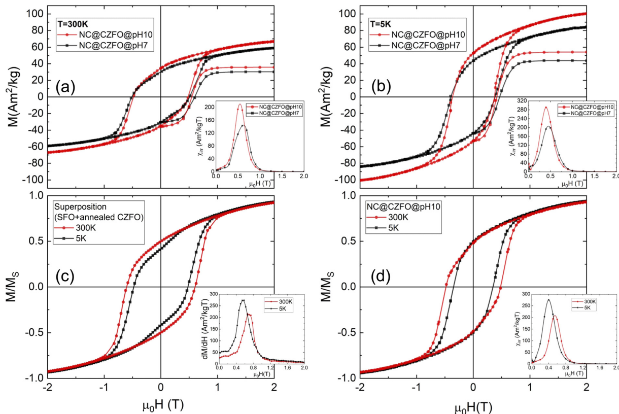
Fig. 6 Magnetization M vs. magnetic field \mu_0 H curves for NC@CZFO@pH10 and NC@CZFO@pH7 and magnetization M_{\text{OCD}} vs. reverse magnetic field \mu_0 H curves for the corresponding samples at (a) 300 K and (b) 5 K. In the insets, the associated SFDs. Normalized magnetization M vs. magnetic field \mu_0 H curves for (c) superposition of CZFO (annealed at the desired temperature) and SFO@pH10 and (d) NC@CZFO@pH10, at both 300 and 5 K. In the insets, the corresponding switching field distributions.
