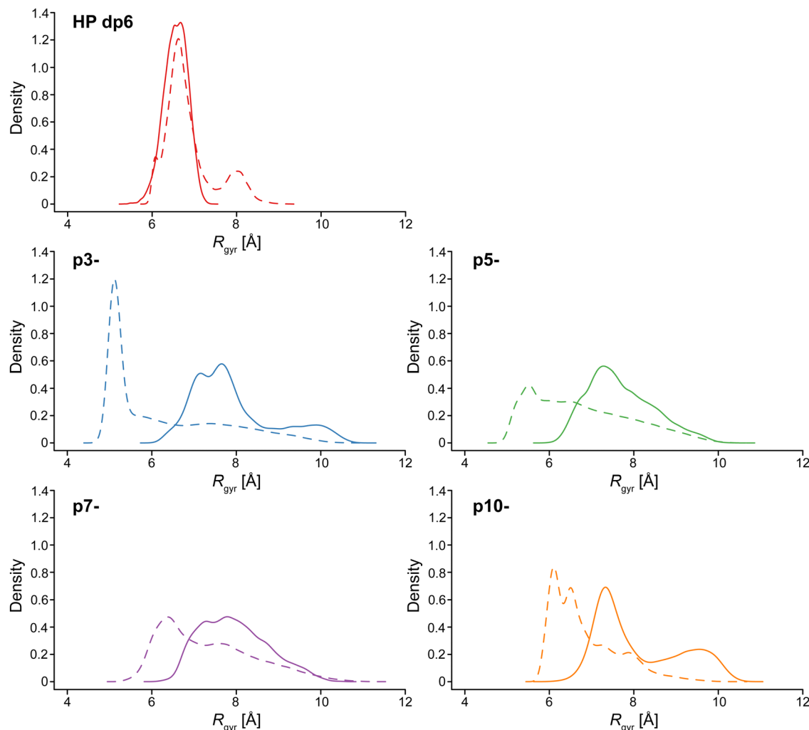
Fig. 9 Comparison of distributions of R_{gyr} values (kernel density estimation) between bound and unbound states in continuous and dashed lines, respectively, for HP dp6, p3-, p5-, p7-, and p10-.
