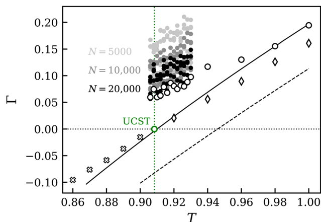
Fig. 9 Thermodynamic factor around the UCST (green circle) of mixture C at p = 0.0724 and x_1 = 0.5 . Results from predictive (dashed line) and adjusted EOS (solid line) 41 have a linear slope below and above the UCST. Simulation results were obtained from chemical potential data below (crosses) and above the UCST (diamonds). KBI results are depicted as a shaded point-cloud (●) for three system sizes. Results for N = 20\,000 based on RDF vdV + shf and extrapolated (white circles) were extended further into the homogenous region.
