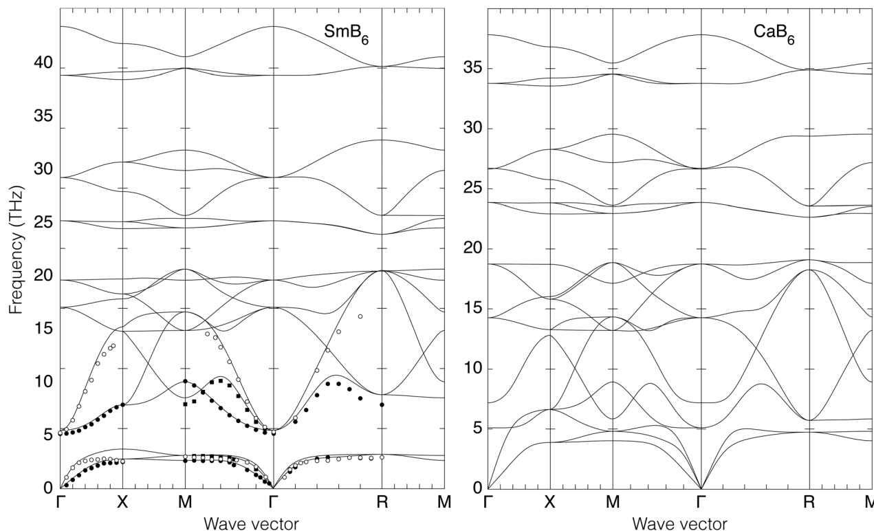
Fig. 4 Calculated phonon dispersion curves of SmB 6 (left) and CaB 6 (right). The wave vector labels have conventional meaning: \Gamma represents the wave vector (0, 0, 0), X represents (\frac{1}{2}, 0, 0) , M represents (\frac{1}{2}, \frac{1}{2}, 0) and R represents (\frac{1}{2}, \frac{1}{2}, \frac{1}{2}) . Results from a single-crystal neutron inelastic scattering experiment 37 are represented as points, using different symbols to aid clarity.
