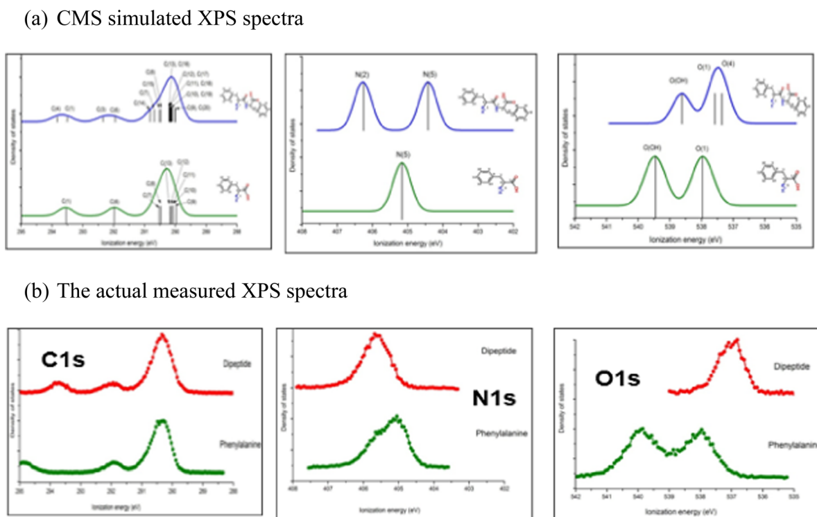
Fig. 9 (a) The CMS simulated C1s, N1s and O1s spectra of phenylalanine monomer and linear phenylalanyl–phenylalanine (dipeptide) and (b) the actually measured XPS spectra. 62
