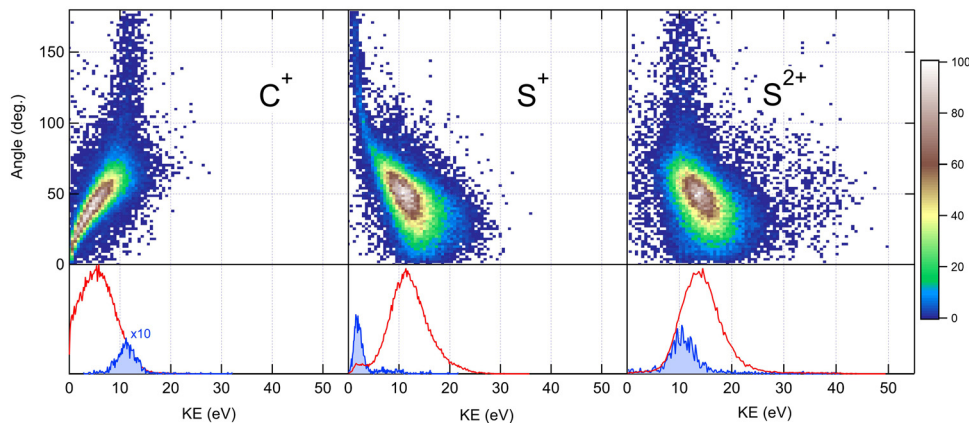
Fig. 6 Angular dependence of the kinetic energy distributions measured for the three fragment ions produced in the dissociation of \text{CS}^{4+} after core S 1s photoionization in \text{CS}_2 . Bottom panels show the 1D projection of the total kinetic energy distributions in red, and the partial distributions in solid blue for a selected range of angles (see the text for details).
