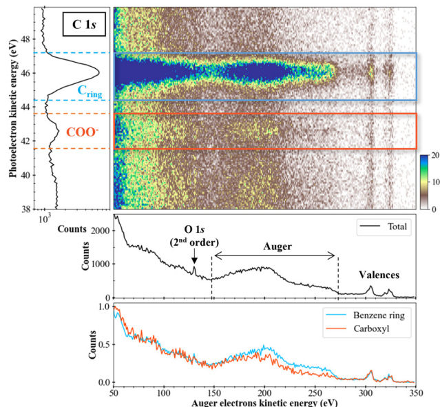
Fig. 5 Two-dimensional map « Auger electrons kinetic energy/photoelectrons kinetic energy » (middle part) in the sodium benzoate case. z -axis was cut at z = 20 counts (with z_{\text{max}} = 71 coincidence counts). Photoelectron spectrum is given on the left, with a step of 0.1 eV. Total (unfiltered) Auger electron spectrum (lower part, in black) is represented with a step of 1 eV. Filtered Auger spectra after photoelectrons emission from carbons of the benzene ring (in blue) and carboxyl group (in orange) are also given. For easier comparison, those spectra are normalized to their maximum.
