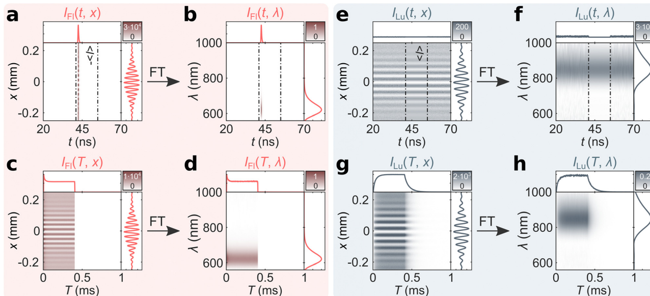
Fig. 3 Fluorescence and luminescence gated bmTG-FTS data of (\text{DNA})_2\text{Ag}_{18}^{12+} . Fluorescence gated (a) mTRIM, (b) mTREM, (c) MTRIM, and (d) MTREM. Luminescence gated (e) mTRIM, (f) mTREM, (g) MTRIM, and (h) MTREM. \langle I \rangle represents the mean luminescence intensity outside the fluorescence time gate. 16
