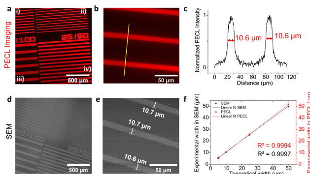
Fig. 2 (a) PECL imaging of n-Si/SiO x patterned with Ir microbands of different width/pitch (i: 10/50 μm; ii: 5/50 μm; iii: 50/100 μm and iv: 25/50 μm – the first and second values refer to the width and the pitch, respectively) at 0.8 V (vs. Ag/AgCl) in PBS 0.1 M solution (pH 7.4) containing 5 mM [Ru(bpy) 3 ] 2+ and 0.1 M TPrA. Exposure time t_{\text{expo}} = 1.5 s. (b) PECL images of the 10/50 μm microbands (as (i) in a) at a higher magnification. (c) Cross-section PECL intensity profiles extracted along the yellow line displayed in (b) with FWHM measurement of the patterns. (d) SEM picture of n-Si/SiO x with Ir microbands as in (a). (e) Zoom on the 10 μm/50 μm microbands recorded by SEM. (f) Comparison of the microband width measured by SEM and PECL imaging (3 measurements for each point).
