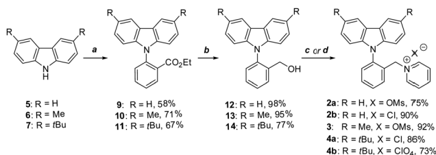
Fig. 2 Synthesis of \text{Py}^+ salts 2–4 . Reagents and conditions: (a) ethyl 2-bromobenzoate ( 8 , 1.2 or 1.3 equiv.), \text{CuI} (15 mol%), L-proline (30 mol%), \text{K}_2\text{CO}_3 , and DMSO, at 140 °C, for 72 h, and a 58% yield for 9 ; 71% for 10 ; and 67% for 11 . (b) \text{LiAlH}_4 , THF, at 70 °C, for 1 h, and a 98% yield for 12 ; 95% for 13 ; and 77% for 14 . (c) \text{MsCl} , DIPEA, and DCM, at 0 °C to rt, for 1 h, then pyridine, MeCN, for 72 h, and a 75% yield for 2a ; 92% for 3 . (d) Conditions (c) followed by reversed-phase chromatography, containing aqueous HCl as a mobile phase, a 90% yield for 2b , and an 86% yield for 4a ; alternatively aqueous \text{HClO}_4 as a mobile phase, 73% yield for 4b .
