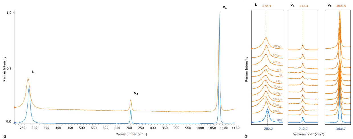
Fig. 2 Comparison among individual Raman spectra of carbonate samples, normalized to the \nu_1 intensity: geogenic calcite (in blue, MAR sample) and anthropogenic calcite (in orange, SFC1L1 sample) (a). Raman spectra details for the anthropogenic sample (in orange) are shown with the geogenic sample (b). Band positions of L, \nu_4 , \nu_1 are reported to highlight the Raman shift, especially in L vibrational mode. Bottom, characteristic values of the band position of the MAR sample (blue), and top, characteristic values of the SFC1L1 sample (first orange band).
