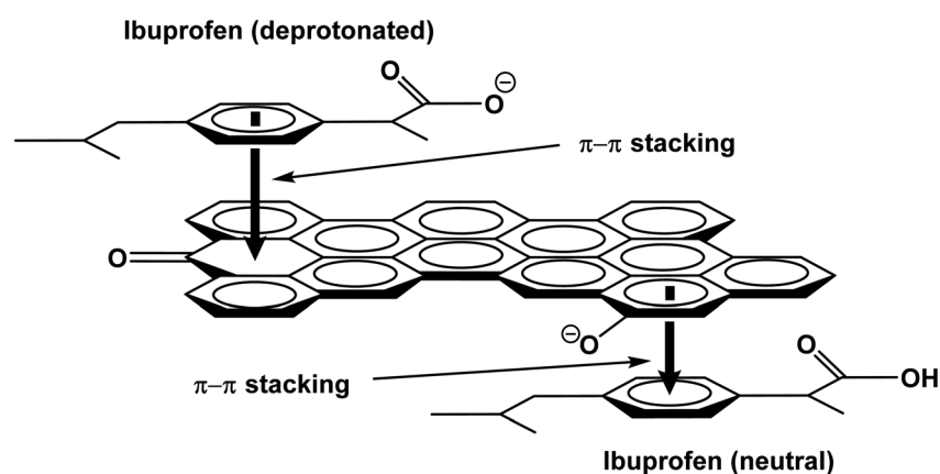
Scheme 6 π–π electron donor–acceptor attractions between neutral and deprotonated ibuprofen with aromatic rings on the WSAB surface.
