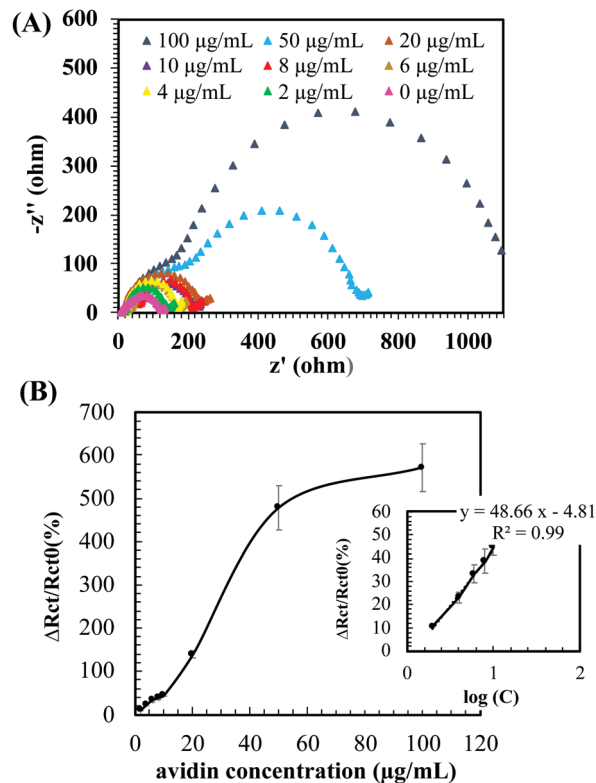
Fig. 7 (A) Impedance Nyquist plots of the EIS from ITO modified with PG/b-pSBAE ( 8/30 \text{ mg mL}^{-1} ) after immersion in avidin solution at various concentrations ( 0 – 100 \mu\text{g mL}^{-1} ). Measurements were performed in PBS containing 10 \text{ mM } [\text{Fe}(\text{CN})_6]^{3-/4-} and 0.1 \text{ M KCl} . (B) Changes in the charge transfer resistance [ \Delta R_{ct}/R_{ct0} (%)] of the PG/b-pSBAE modified ITO after immersion in avidin solution at various concentrations. Insert: the corresponding regression curve of the PG/b-pSBAE modified ITO. C: Avidin concentration. Value = mean \pm standard deviation, n = 3 .
