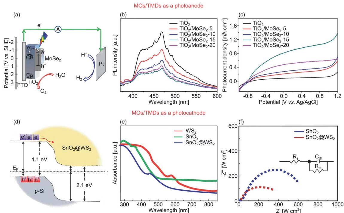
Fig. 11 (a) A diagram of PEC water splitting using \text{TiO}_2/\text{MoSe}_2 photoanode under visible light. (b) Photoluminescence spectra and (c) polarization curves of \text{TiO}_2 , \text{TiO}_2/\text{MoSe}_2 -5, \text{TiO}_2/\text{MoSe}_2 -10, \text{TiO}_2/\text{MoSe}_2 -15, and \text{TiO}_2/\text{MoSe}_2 -20. The number represent the amount of \text{MoSe}_2 loading, 5 (2 mM \text{MoSe}_2 ), 10 (4 mM \text{MoSe}_2 ), 15 (6 mM \text{MoSe}_2 ), and 20 (8 mM \text{MoSe}_2 ). (d) Band positions and carrier motion of \text{SnO}_2/\text{WS}_2 photocathode to generate hydrogen under visible light. (e) UV-visible absorption and (f) EIS Nyquist plot of \text{SnO}_2/\text{WS}_2 photocathode with 0.06 M of \text{WS}_2 loading, and its constituent controls. Figures adapted with permission from: (a–c) ref. 77. Copyright 2019 Wiley-VCH. (d–f) Ref. 78. Copyright 2019 American Chemical Society.
