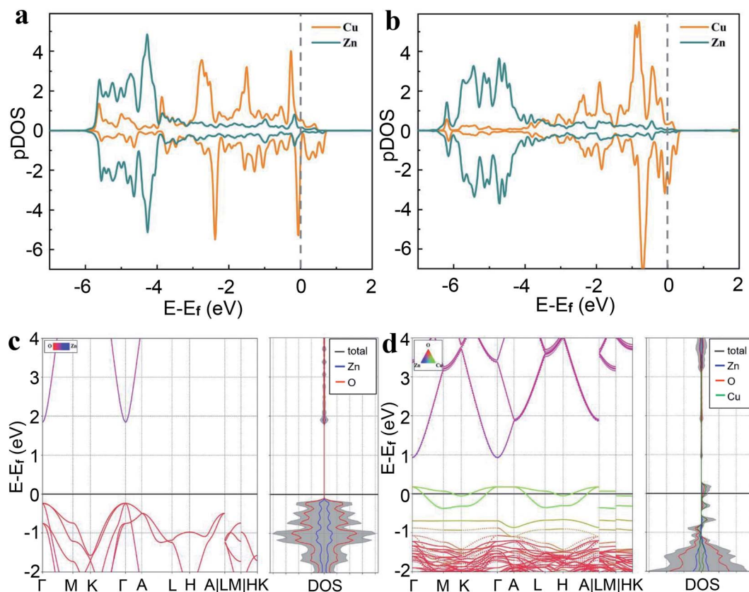
Fig. 5 Projected density of state (pDOS) of surface Zn and Cu atoms in (a) doped \text{Cu}_1@ZnO model (Fig. 4b), and (b) supported \text{Cu}_1/ZnO model (Fig. 4c). Band structure of (c) pure ZnO and (d) doped \text{Cu}_1@ZnO in which one Zn atom in the 2 \times 2 \times 2 supercell of ZnO is replaced by one Cu atom.
